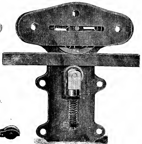
Fig. 2829. HATFIELD HANGING-DOOR SHEAVE. (Used for both passenger and freight cars.)
